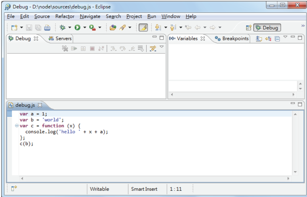
图3-15 Debug perspective
