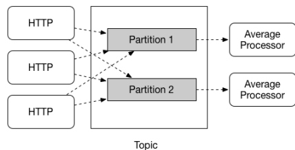
图8. Spring Cloud Stream分区
