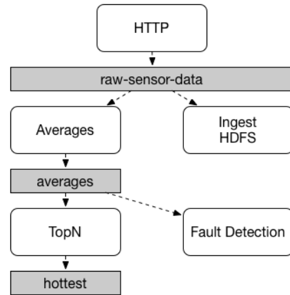
图6. Spring Cloud Stream Publish-Subscribe
