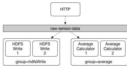
图7. Spring Cloud Stream消费者组
