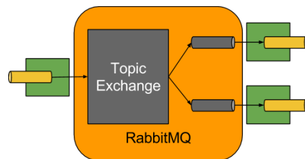
图14. RabbitMQ Binder
