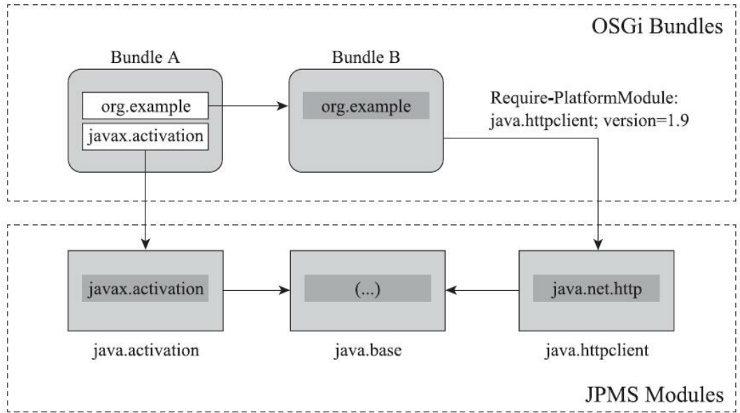
图7-4 OSGi与JPMS交互 [4]
